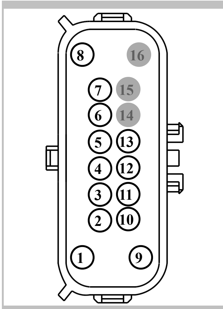
MALE Harness 14D230
