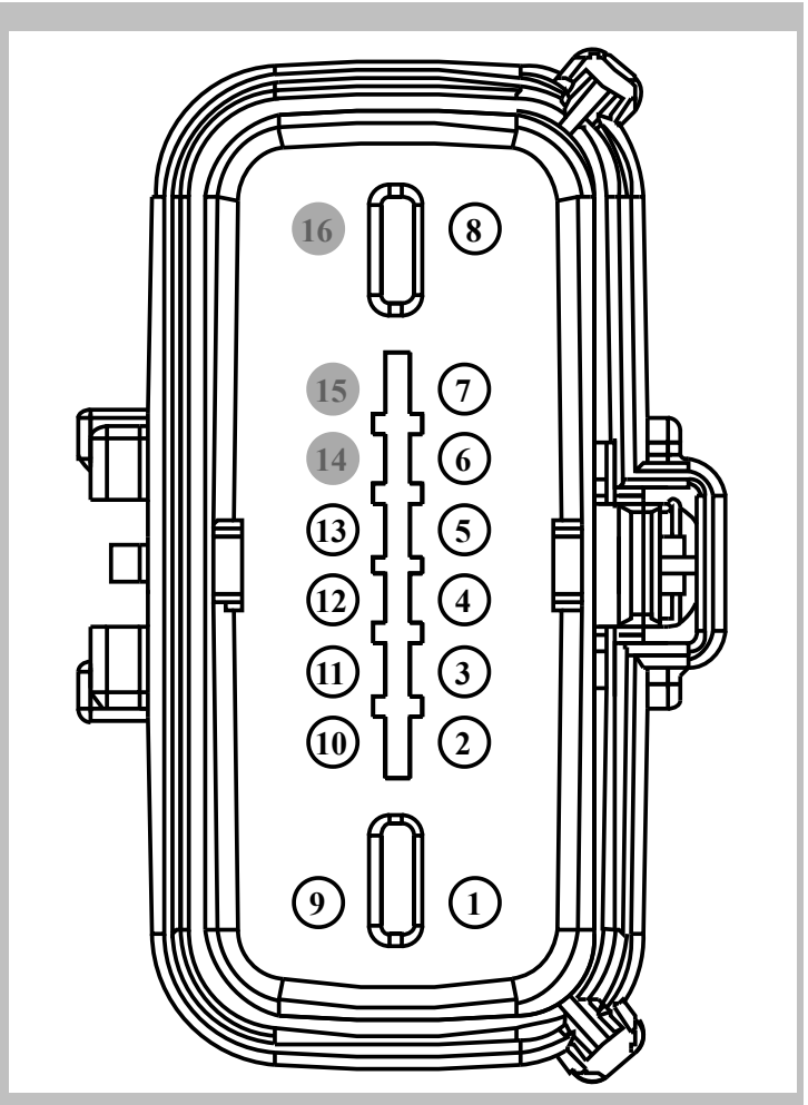
FEMALE Harness 14A005
